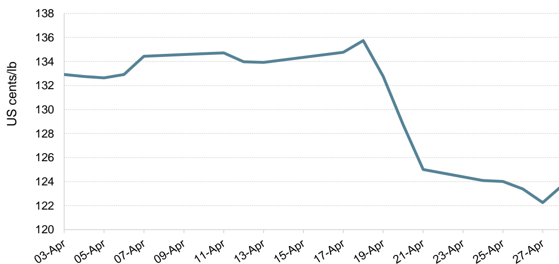
ICO composite indicator price - April 2017
